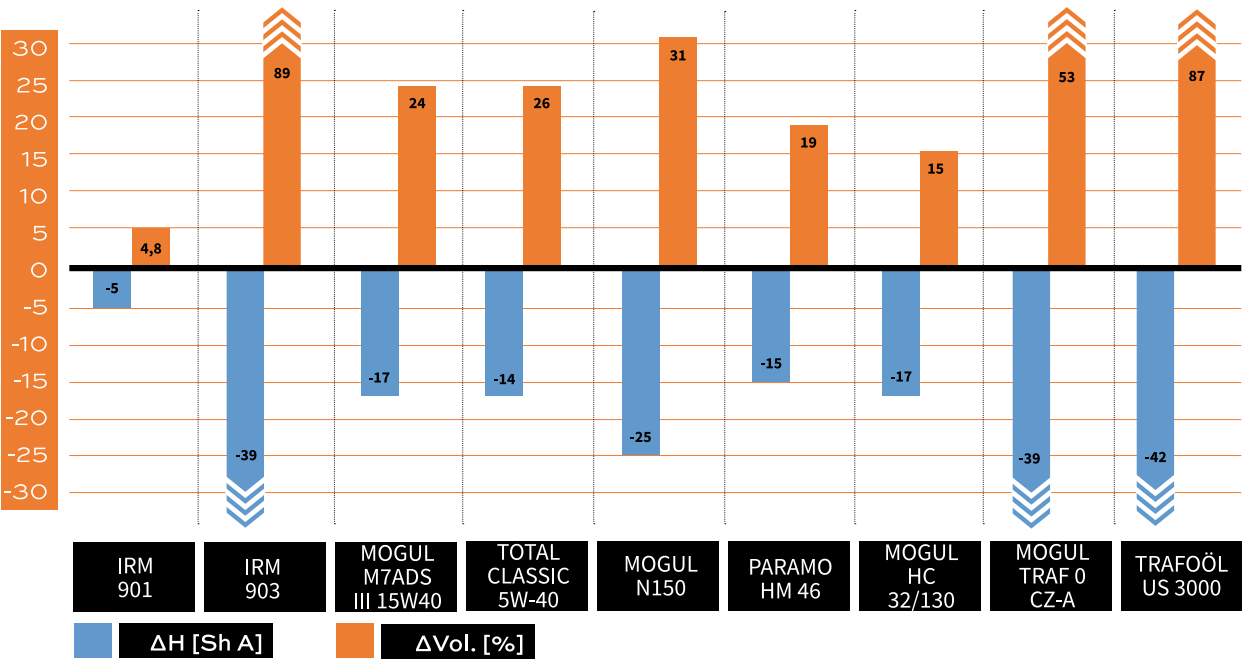
7645 SWELLING RATES
